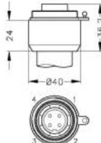
Bussaneer (IP 68) 9
